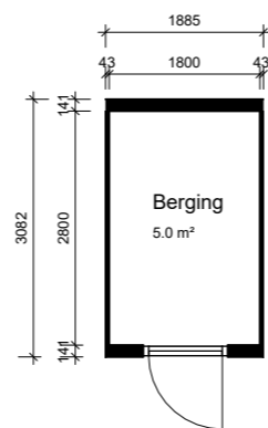
begane grond - berging
