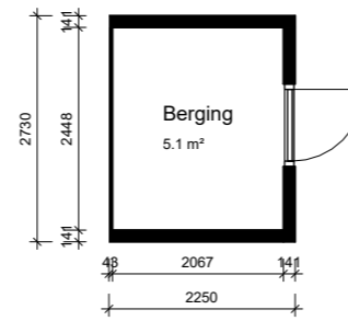
begane grond - berging
