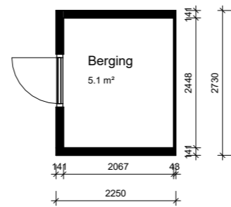
begane grond - berging
