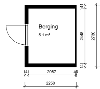
begane grond - berging
