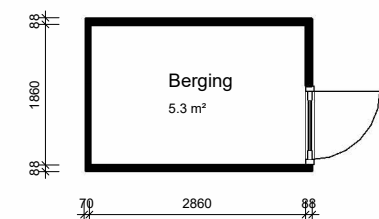
berging
